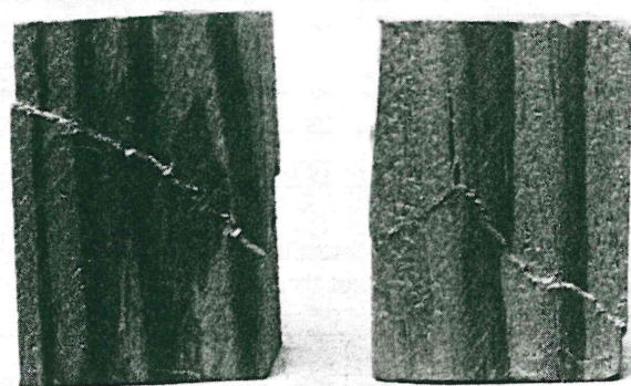
Fig. 2. Typical failure patterns for test cores (diameter of 15 mm) and standard test specimens
