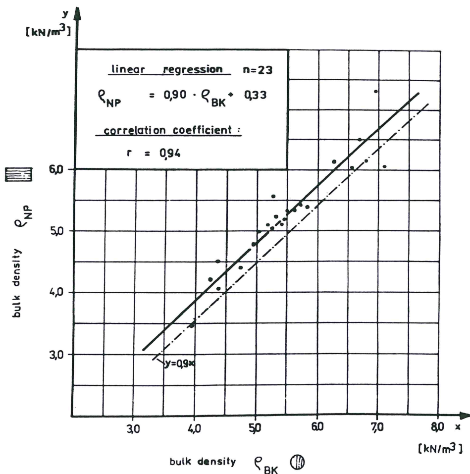
Fig. 5. Comparison of the bulk density of the test cores with the bulk density of the standard test specimens
